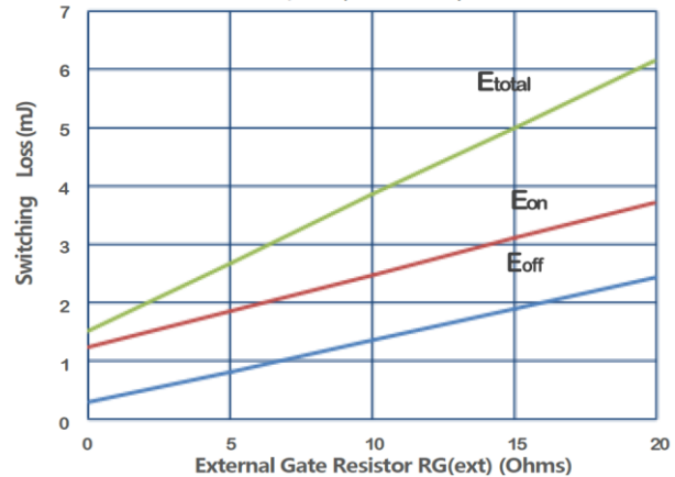
Fig14. Switching Energy vs. RG(ext)
