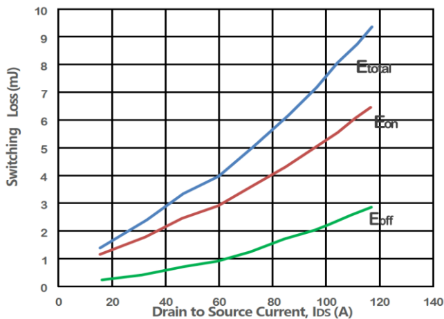
Fig13. Switching Energy vs. Drain Current
