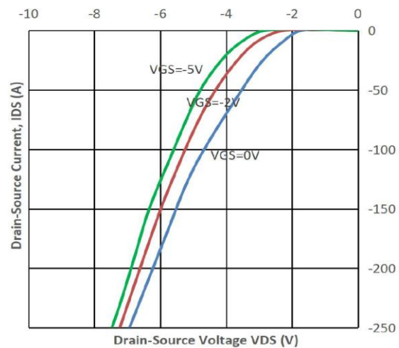
Fig6. Body Diode Characteristic at 25 °C
