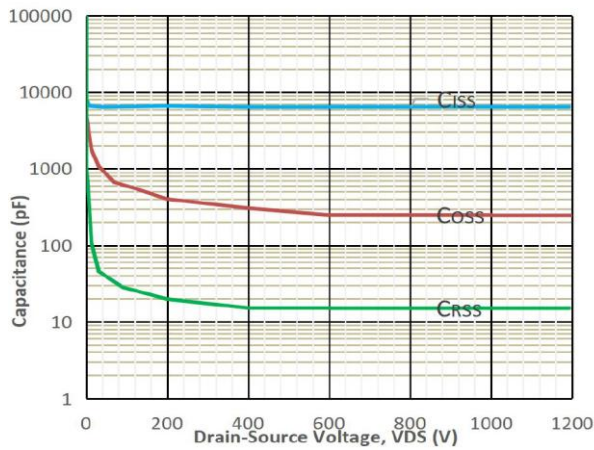
Fig11. Capacitances vs. Drain-Source
