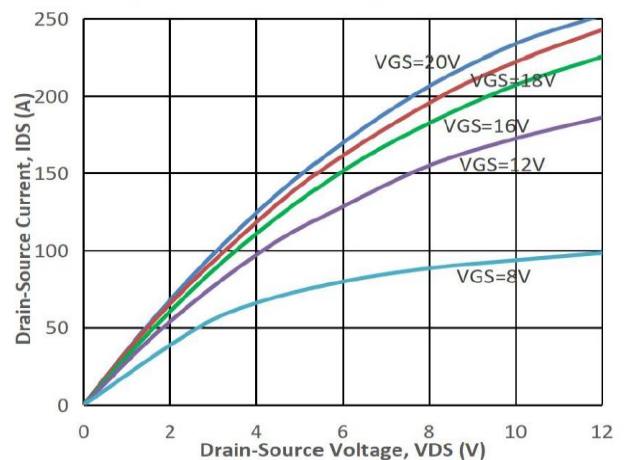
Fig2. Output characteristics ( T_J = 175^\circ\text{C} )
