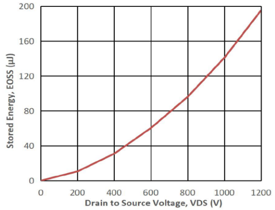
Fig10. Output Capacitor Stored Energy
